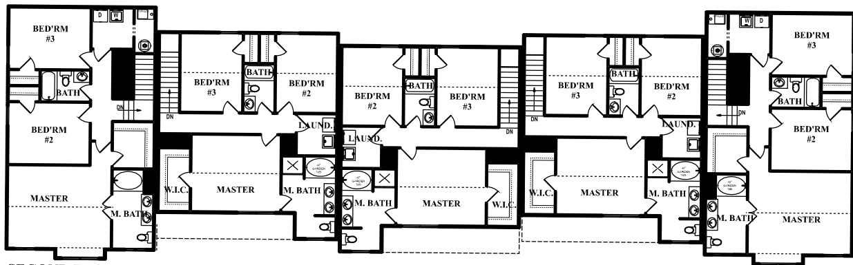
SECOND FLOOR
